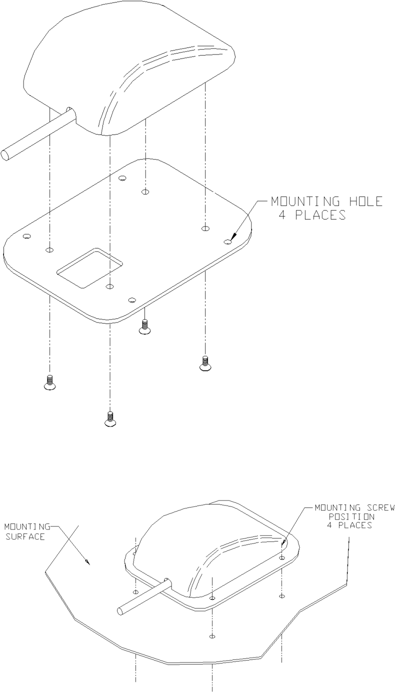
Fig. 6, Flange Mount Attachment
